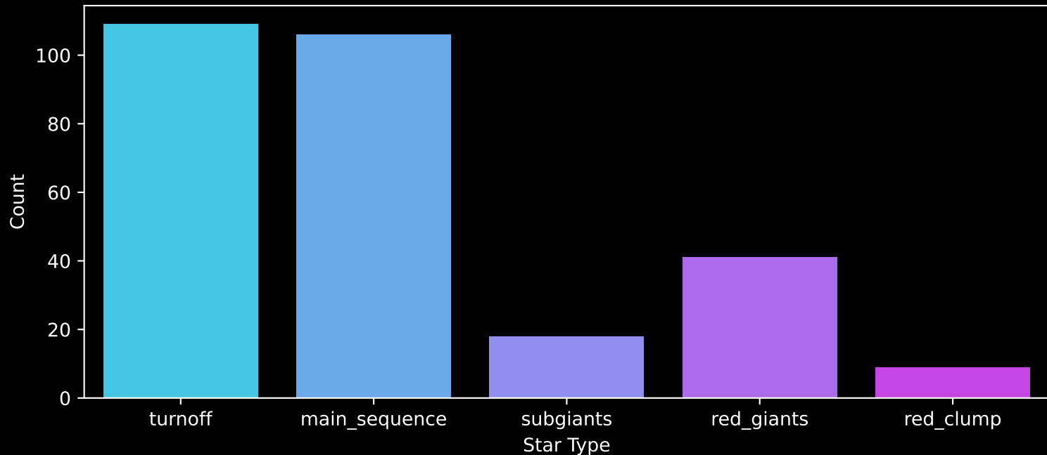
GALAH DR4 Field: [1832] Count plot of Star Type
