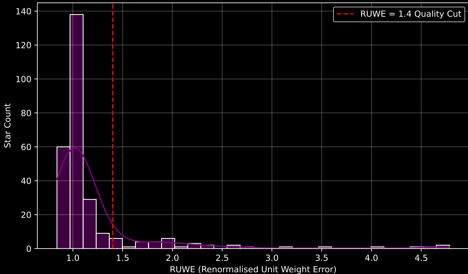
GALAH DR4 Field [1832] RUWE Distribution (n= 273)
